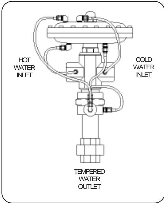
THERM-O-MIX® STATION/WWM Utilizes hot & cold water mixing to produce tempered water supply
