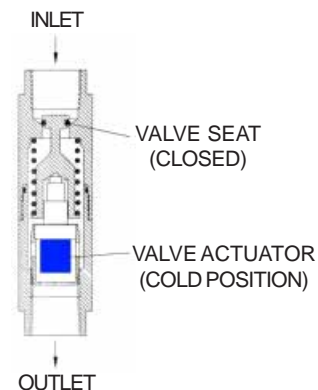
REVERSE ACTING
