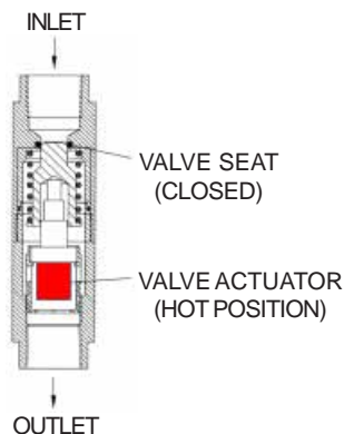
DIRECT ACTING
