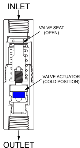
DIRECT ACTING
