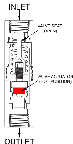
REVERSE ACTING
